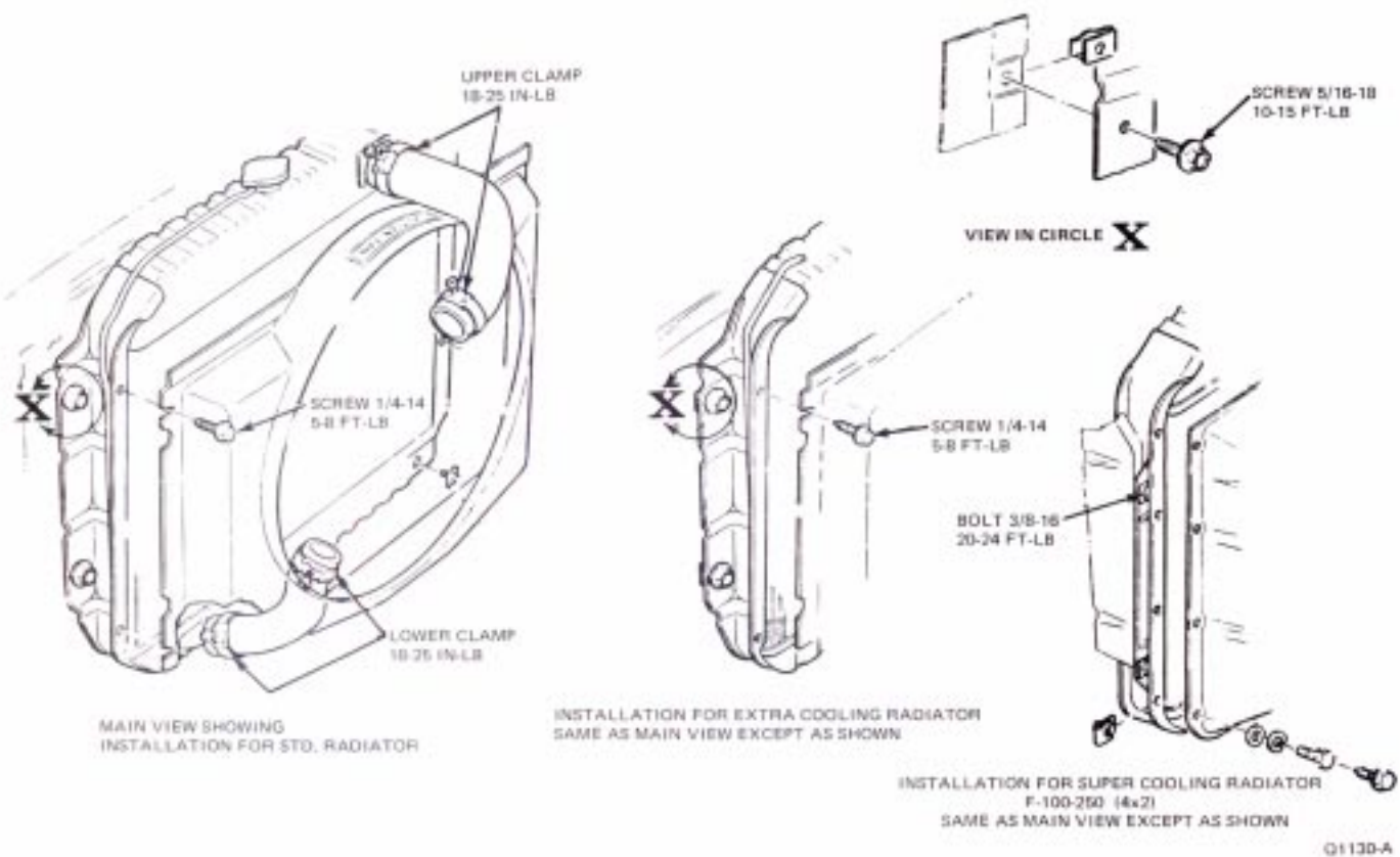
FIG. 7 Radiator Installation—F-100-250-350—8 Cylinder
