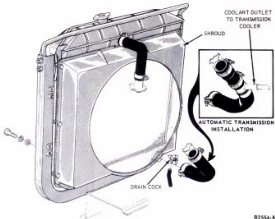
FIG. 6 Radiator Installation—P-Series
