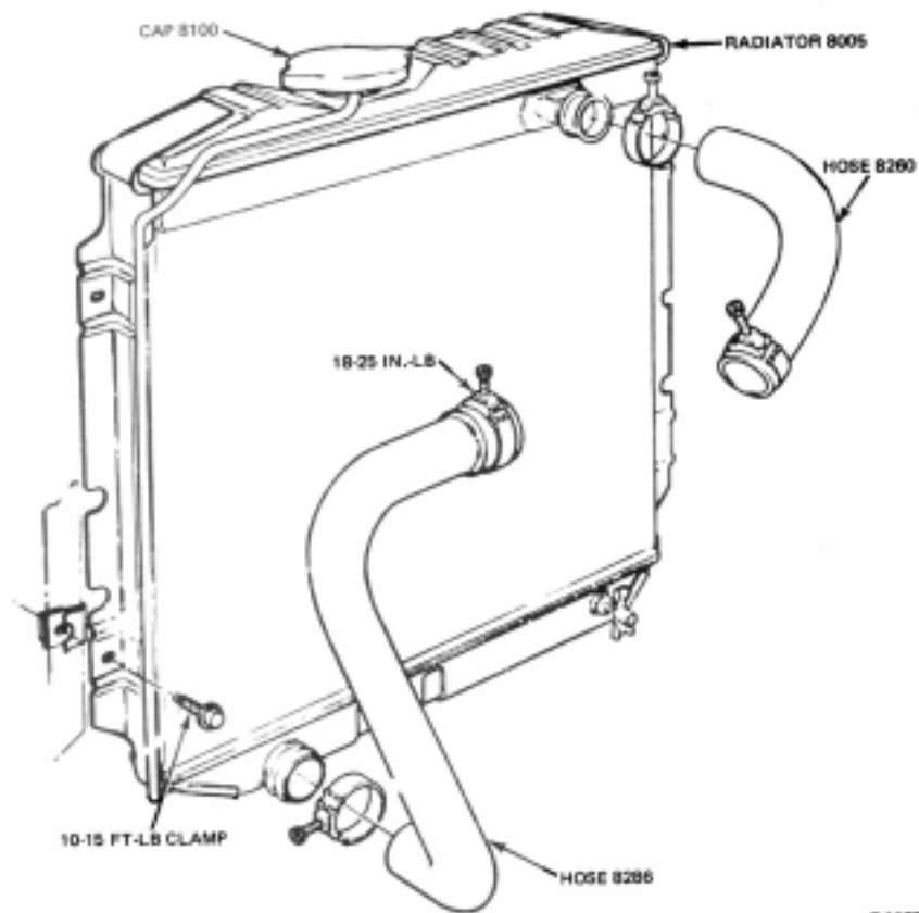
FIG. 5 Radiator Installation—Bronco 6 Cylinder
