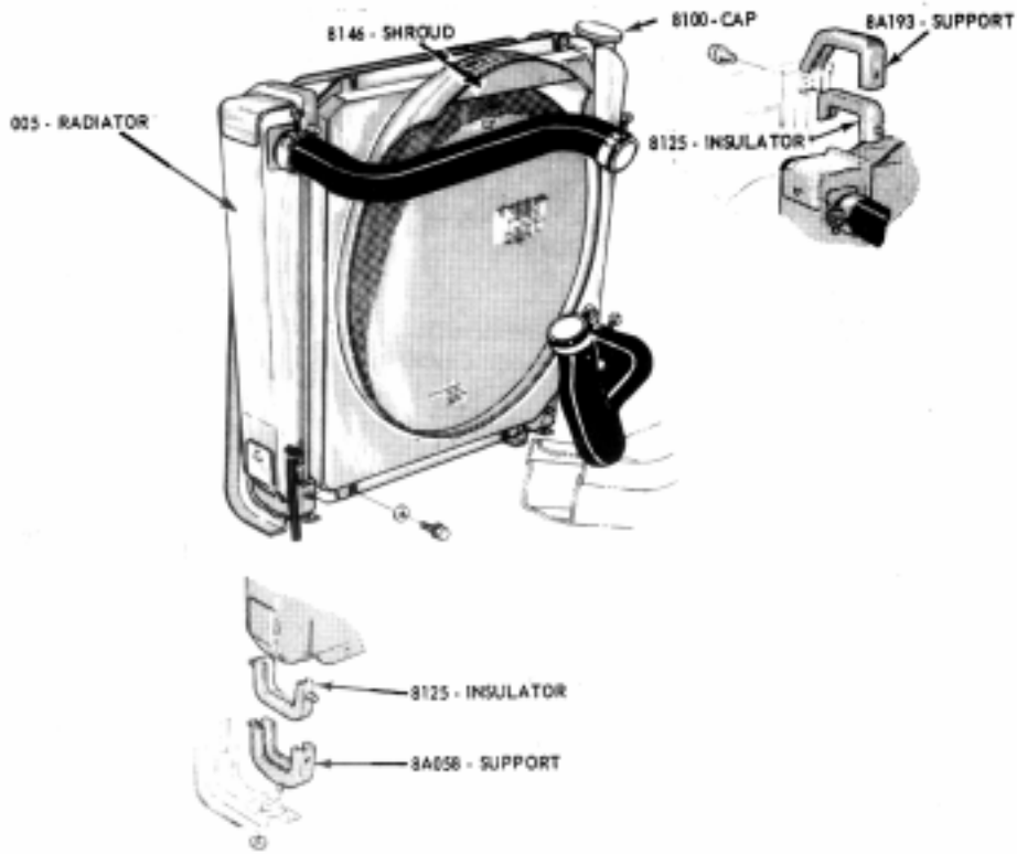
FIG. 4 Radiator Installation—Bronco 8 Cylinder
