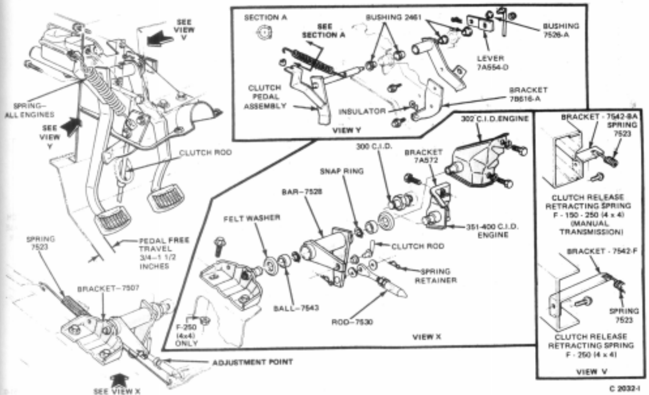
FIG. 4 F-100—F-350 Series Clutch System
