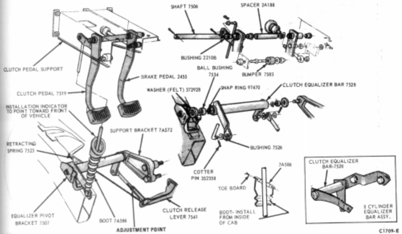
FIG. 3 Clutch Linkage—Bronco
