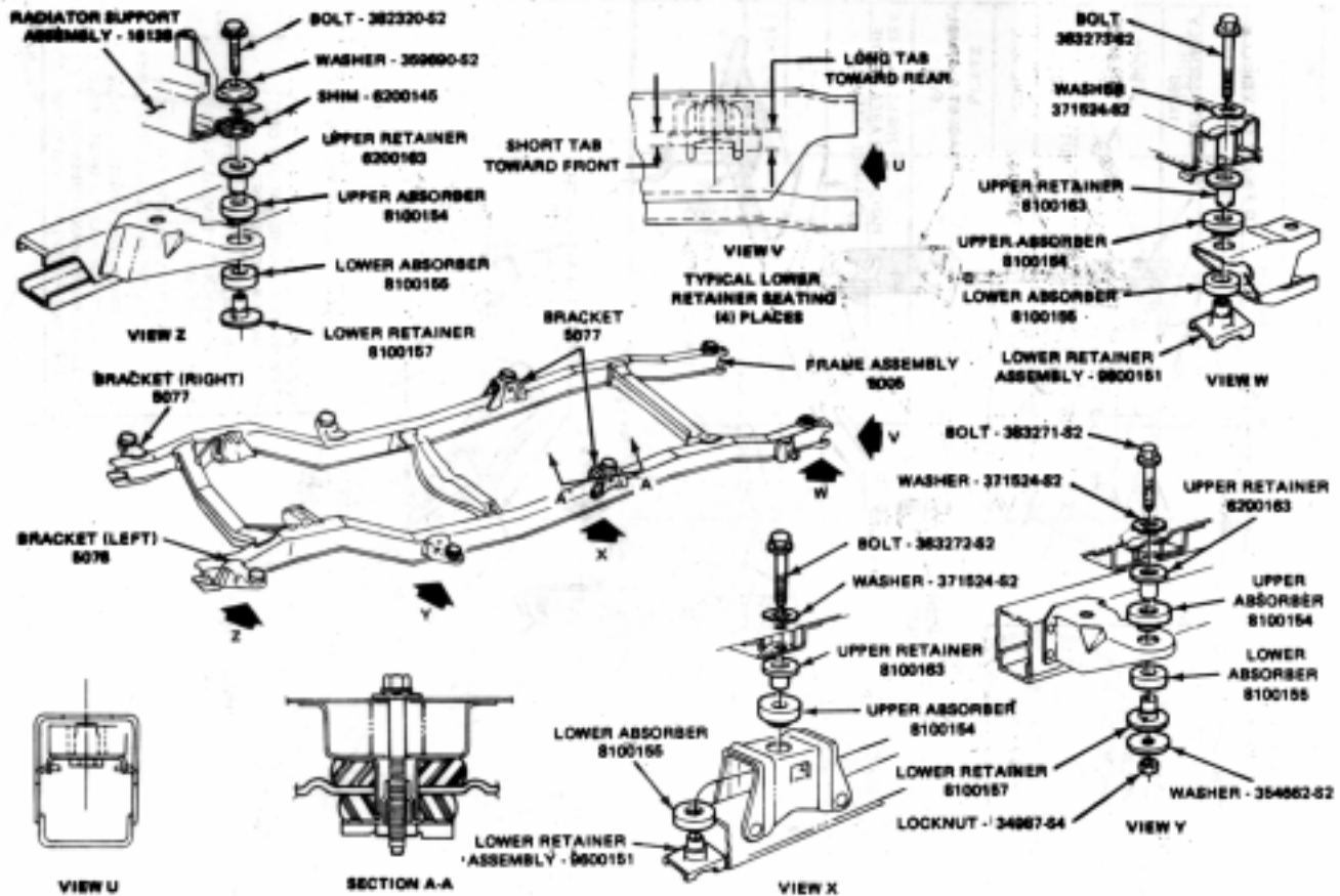
FIG. 13 Body Mounts—Bronco
